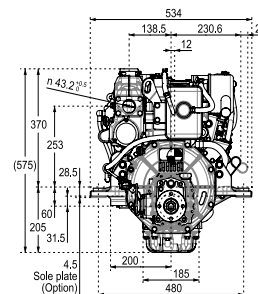
With KM2P-1 gearbox / Rear view
